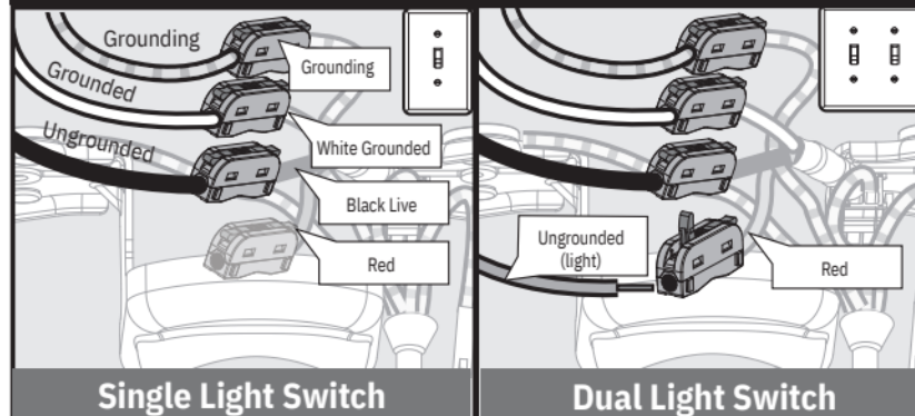
Wiring your bracket depending on single or dual switch
